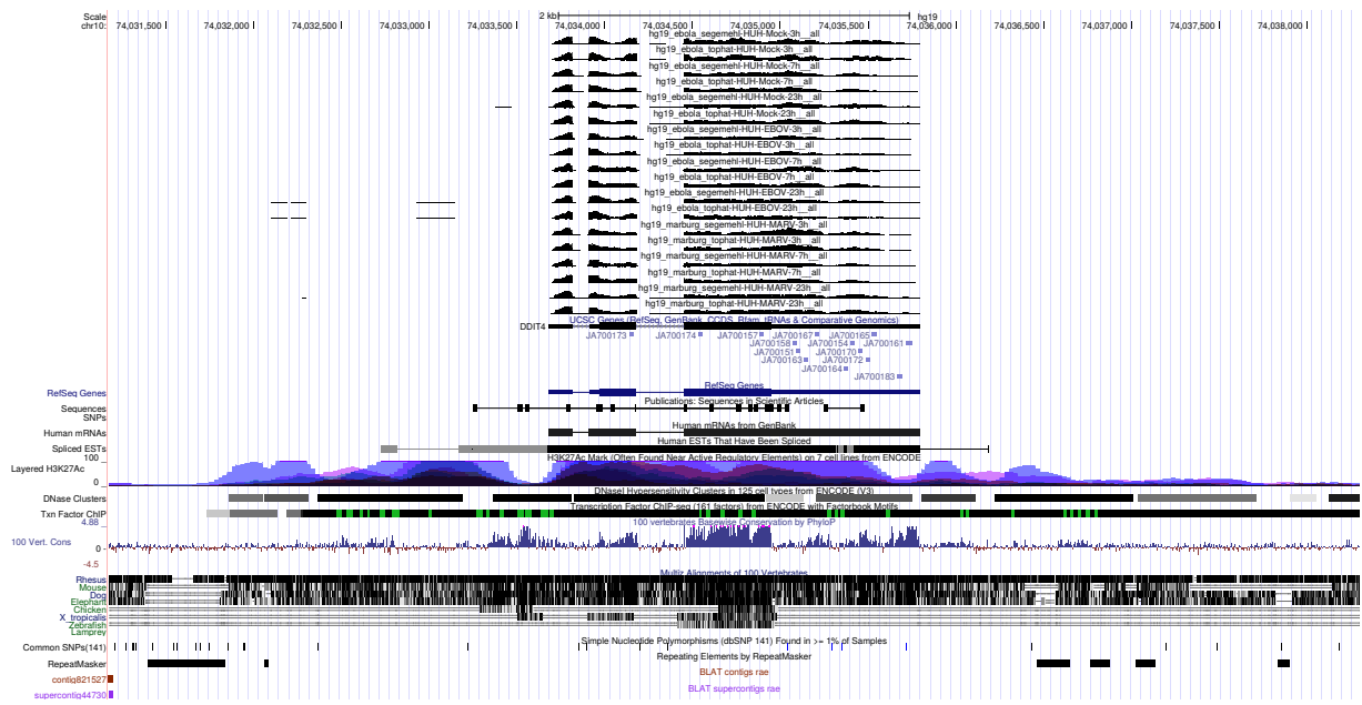
Figure 3: UCSC Genome Browser screenshot of gene DDIT4.
