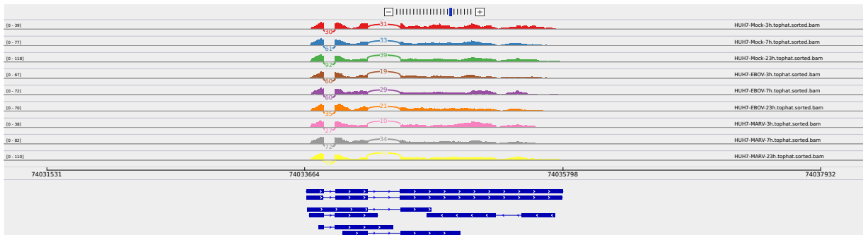
Figure 2: Sashimi plot of gene DDIT4.
