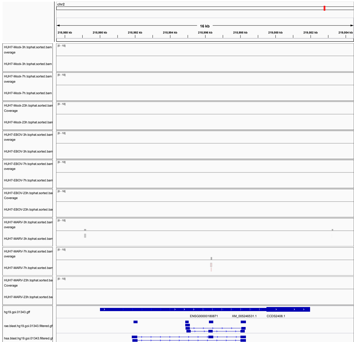
Figure 1: IGV Genome Browser screenshot of gene CXCR2.
