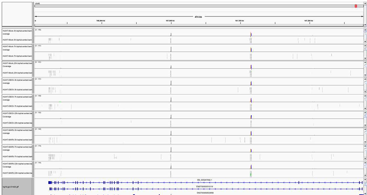
Figure 1: IGV Genome Browser screenshot of gene RPS6KA2.
