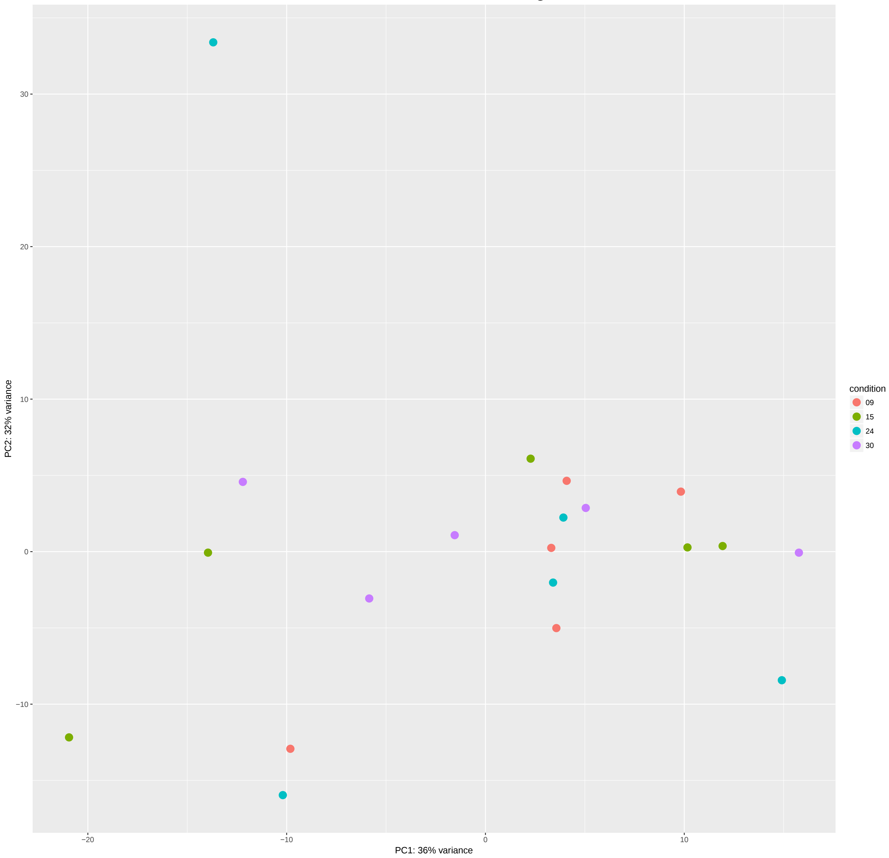
Principal Component Analysis based on the 1000 most variant genes
